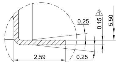
DETAIL "B" S=6
