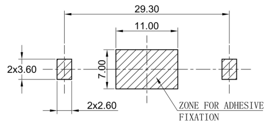
PCB MOUNTING LAYOUT
