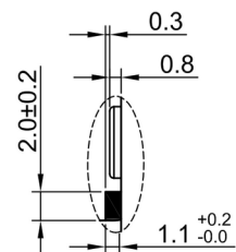
POLARITY PROTECTION DEVICE DETAIL "A" S=2
