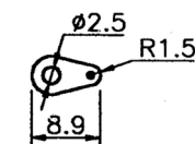
SOLDER
