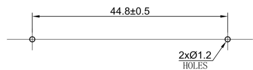
PCB/MOUNTING LAYOUT
