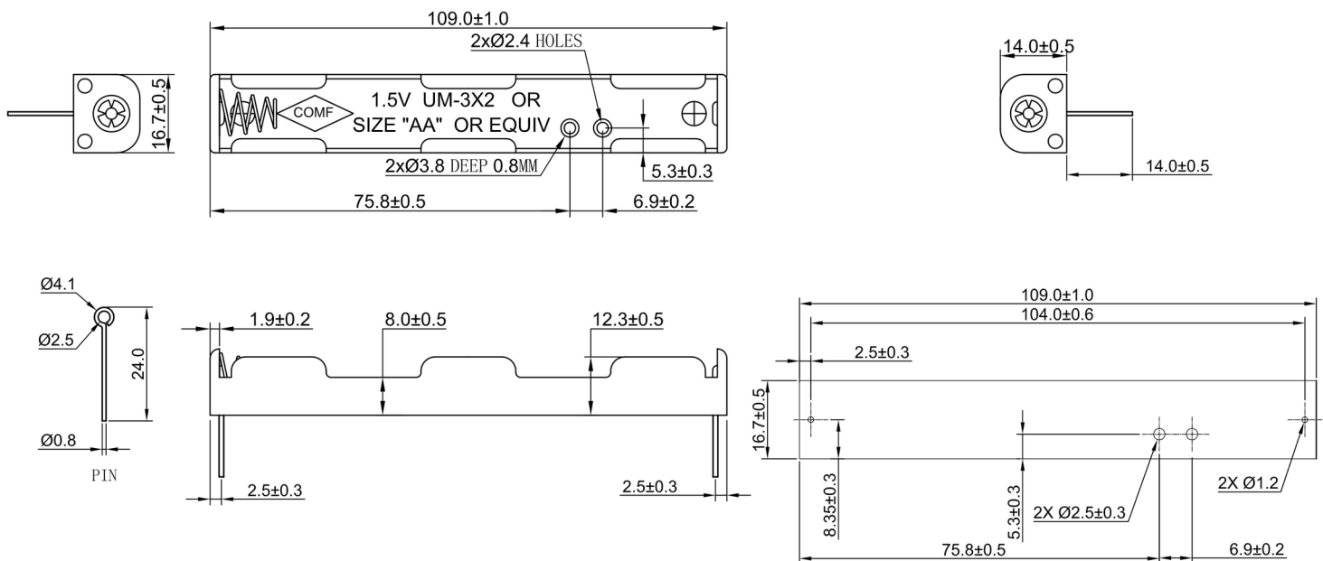
PCB MOUNTING LAYOUT
