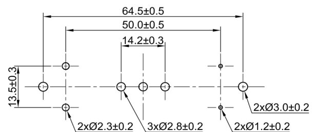
PCB/MOUNTING LAYOUT
